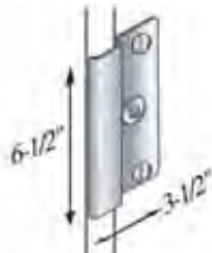
6-1/2" LATCH GUARD Heavy gauge steel 1-1/8" backset Cylinder guard MG-8852AL MG-8852DU
