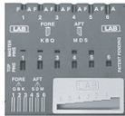
LA-LPDMED MEDECO PIN DECODER AND KEY GAUGE FOR BIAxIAL
