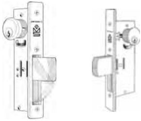
MS1850S MS1850S 220/320
