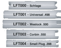
LA-LFT005 PLUG FOLLOWER SET
